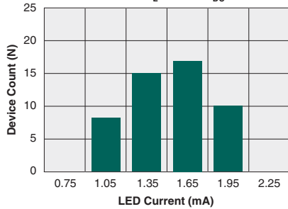
Typical I F for Switch Operation (N=50, I L =350mA DC )
