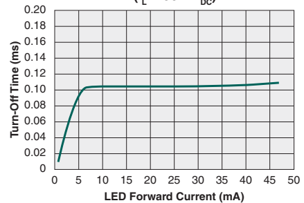
Typical Turn-Off Time vs. LED Forward Current (I L =200mA DC )
