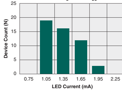
Typical I F for Switch Dropout (N=50, I L =350mA DC )
