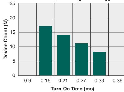
Typical Turn-On Time (N=50, I F =5mA, I L =350mA DC )
