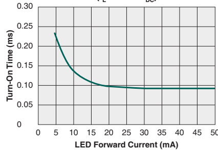
Typical Turn-On Time vs. LED Forward Current (I L =200mA DC )
