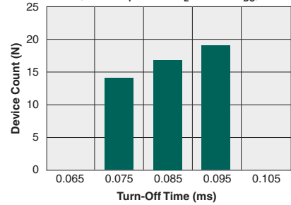
Typical Turn-Off Time (N=50, I F =5mA, I L =350mA DC )
