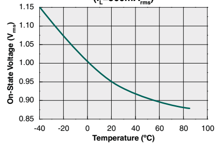
Typical On-State Voltage vs. Temperature ( I_L=500mA_{rms} )
