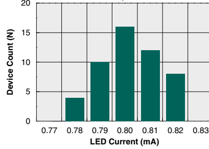
Typical I_F for Switch Operation ( I_L=1A_{rms} , T_A=25^\circ C )
