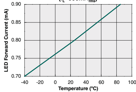
Typical I_F for Switch Operation vs. Temperature ( I_L=500mA_{rms} )
