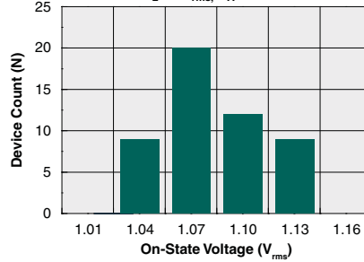
Typical On-State Voltage ( I_L=1A_{rms} , T_A=25^\circ C )
