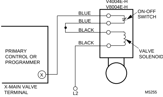
WIRING METHOD 2
