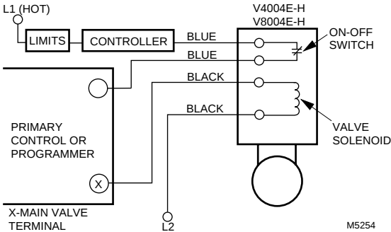
WIRING METHOD 1
