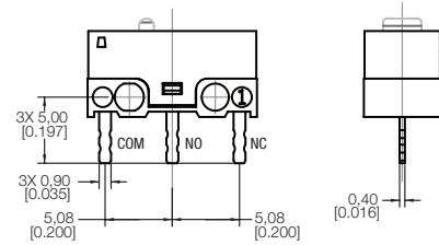
TYPE 20 - PCB STRAIGHT
