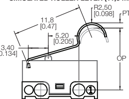
TYPE E SIMULATED ROLLER LEVER (11,8 mm; R2.5)
