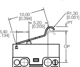
TYPE G SIMULATED ROLLER LEVER(10.0 mm,R1.3)
