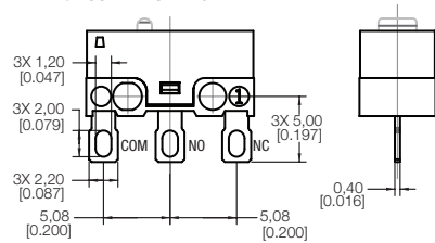
TYPE 10 - SOLDER STRAIGHT
