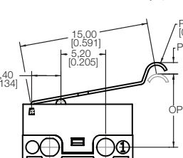
TYPE H SIMULATED ROLLER LEVER (15,0 mm; R1.3)
