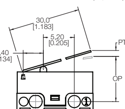
TYPE J LONG STRAIGHT LEVER (30,0 mm)
