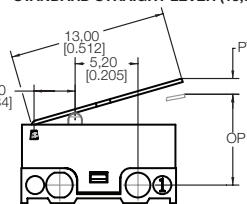
TYPE C STANDARD STRAIGHT LEVER (13,0 mm)
