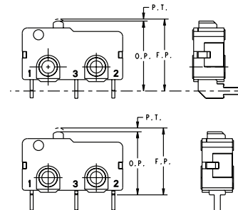
Operate Point References for PCB Terminals
