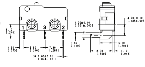
Terminal Type 60 - Left PCB
