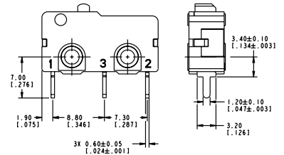
Terminal Type 70 - Long Solder
