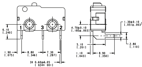
Terminal Type 50 - Right PCB
