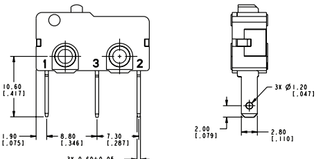
Terminal Type 70 - Long Solder
