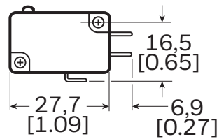
Figure 6. Solder
