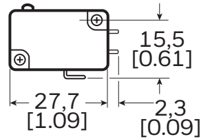
Figure 7. Short Solder
