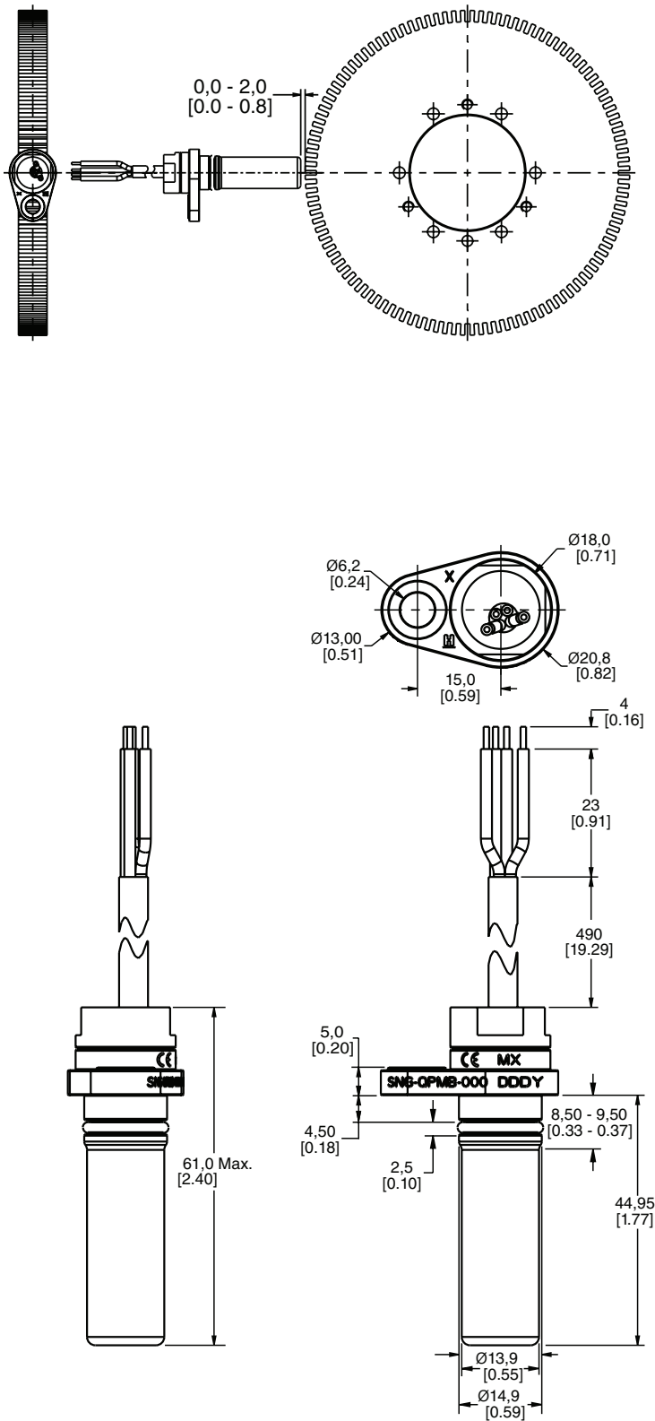
FIGURE 7. SNG-QPMB-000 MOUNTING DIMENSIONS (FOR REFERENCE ONLY: MM/[IN.] )
