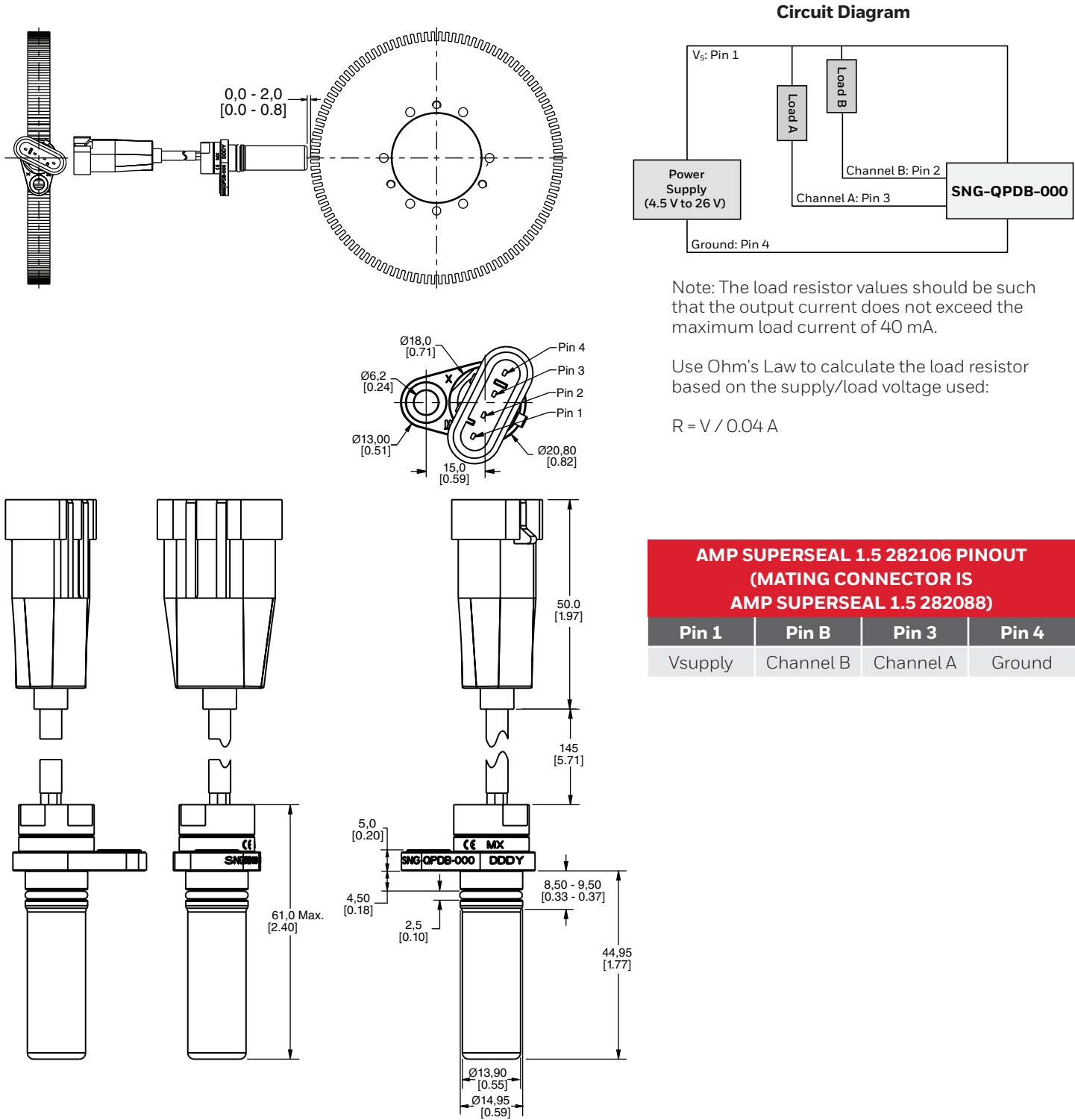
FIGURE 8. SNG-QPDB-002 MOUNTING DIMENSIONS (FOR REFERENCE ONLY: MM/[IN.])
