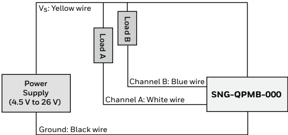
Circuit Diagram
