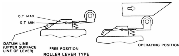
Figure 7 – Roller lever safe travel zone
