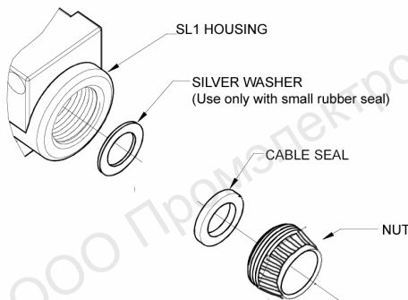
Figure 1 – Cable seal selection
