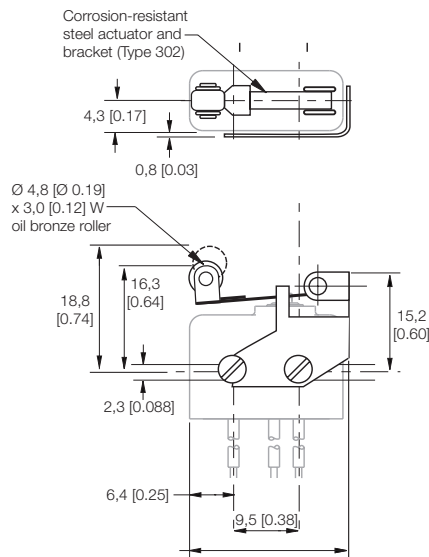
Figure 12. JM-1 Dimensions
