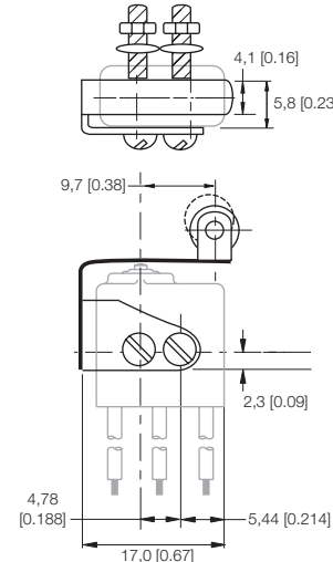
Figure 13. JM-5 Dimensions
