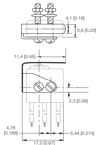
Figure 12. JM-1 Dimensions
