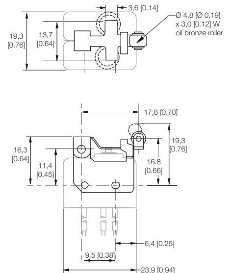
Figure 13. JM-5 Dimensions
