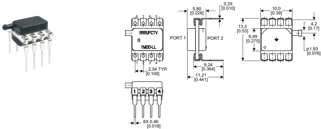
Figure 5. DIP Package Dimensional Drawings (continued)
