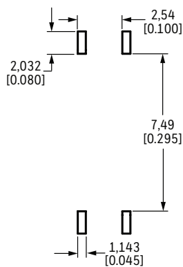
Figure 5. Leadless SMT Package Dimensional Drawings (For reference only: mm [in].)
