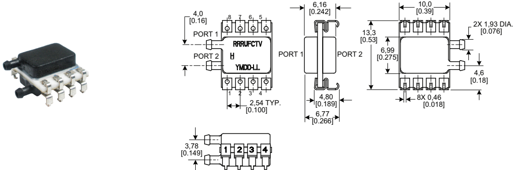
Figure 7. SMT Package Dimensional Drawings (continued)
