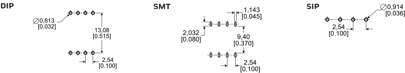
Figure 9. Recommended PCB Pad Layouts
