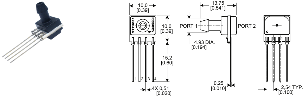
Figure 8. SIP Package Dimensional Drawings (continued)
