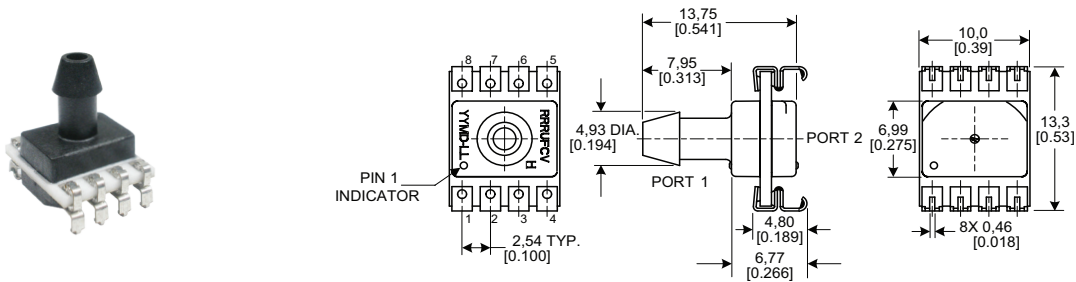
Figure 7. SMT Package Dimensional Drawings (continued)
