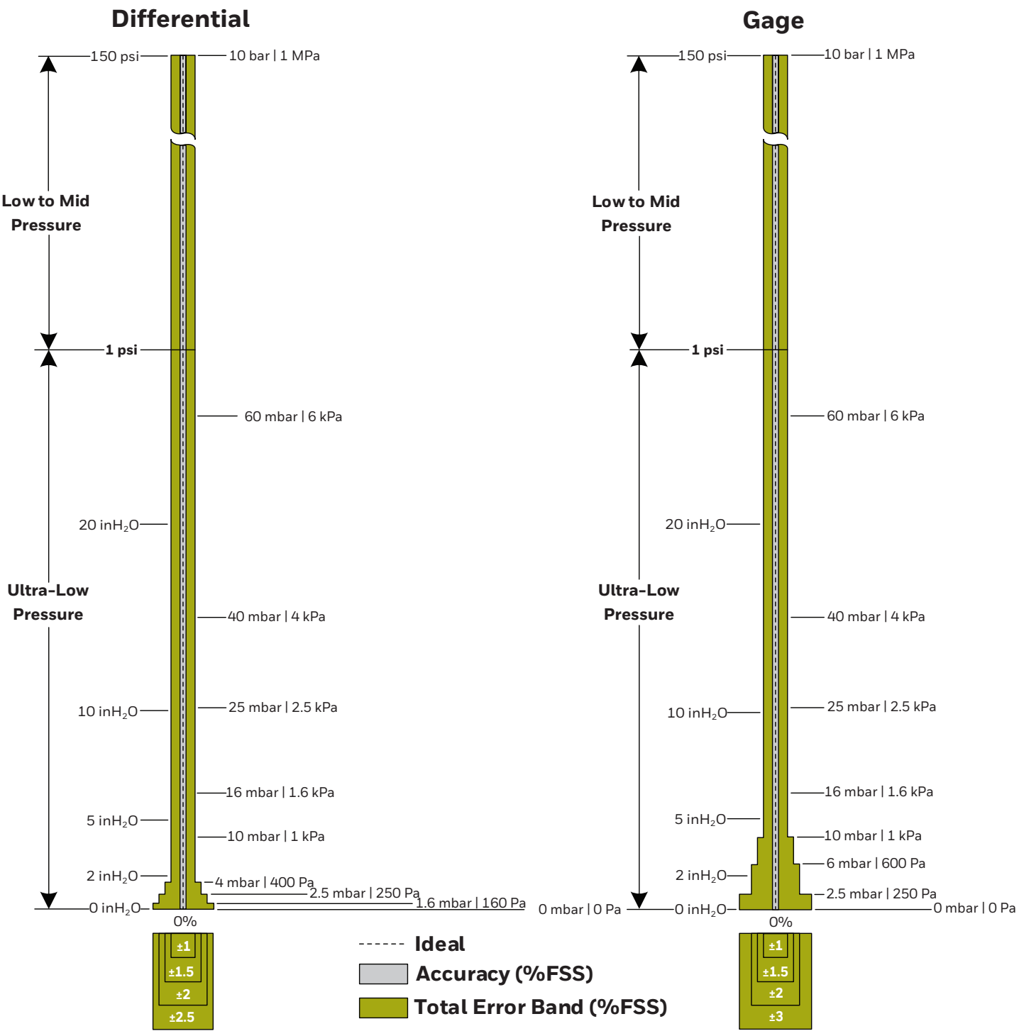
TOTAL ERROR BAND VALUES Figure 3. Total Error Band Values for Full Scale Span Pressure Ranges
