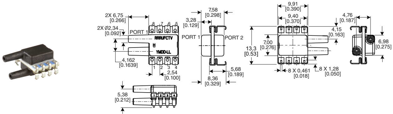
Figure 7. SMT Package Dimensional Drawings (continued) SMT JJ: Dual radial barbed ports, same side
