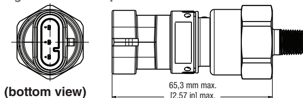
Figure 14. AMP Superseal 1.5
