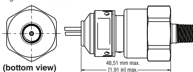
Figure 17. Wire out
