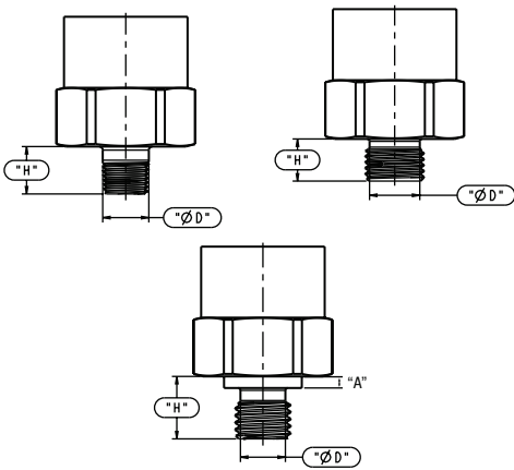
Figure 13. MH Series Pressure Port Dimensions
