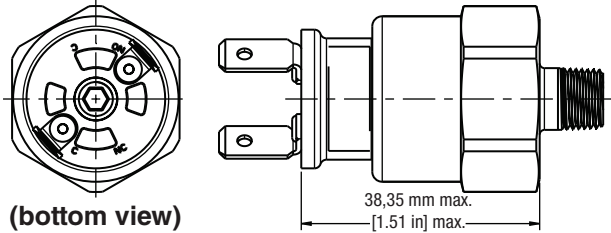
Figure 11. Blade terminal
