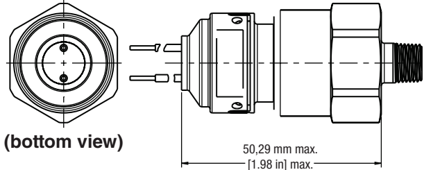
Figure 10. Wire out
