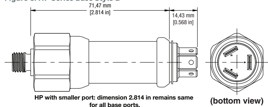
Figure 6. HP Series Base Style B
