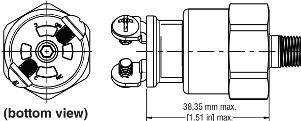
Figure 12. Screw terminal
