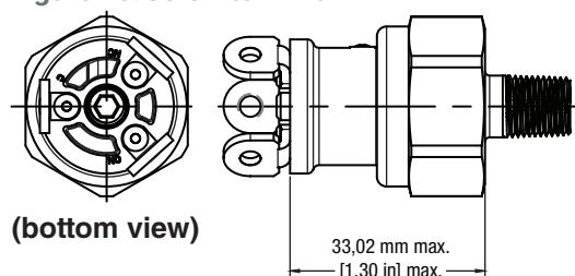
Figure 26. Screw terminal
