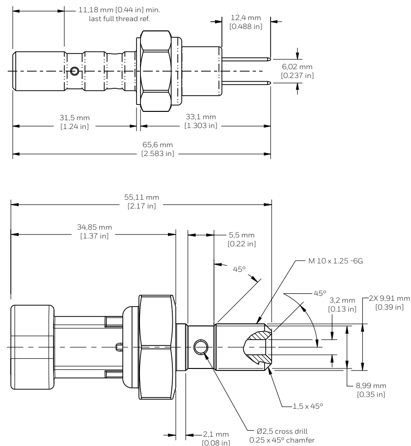
Figure 28. 1000 Series Dimensions
