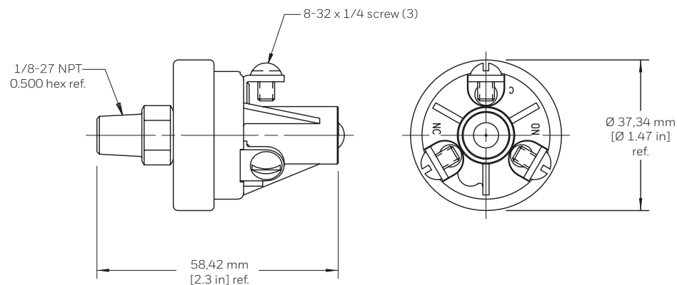
Figure 29. 5000 Series Dimensions
