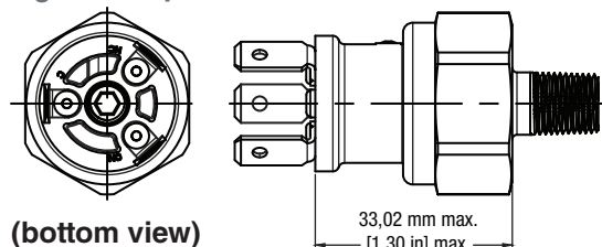
Figure 25. Spade terminal
