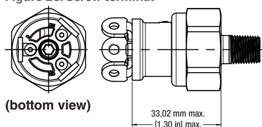
Figure 26. Screw terminal
