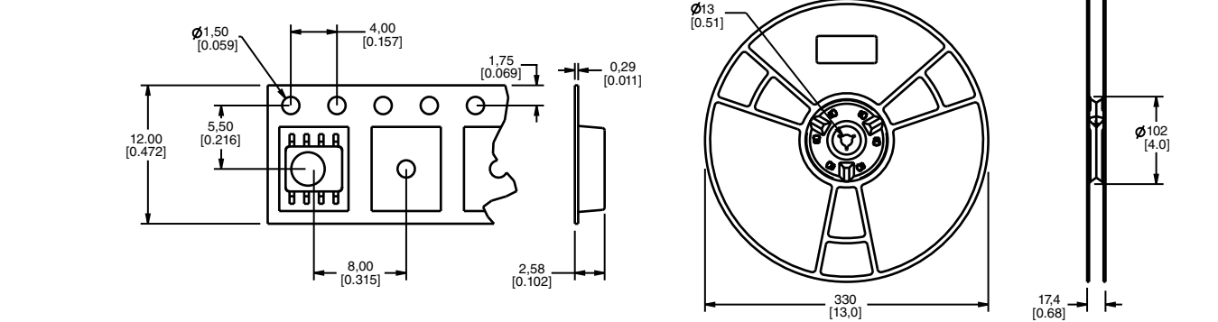
Tape and Reel
