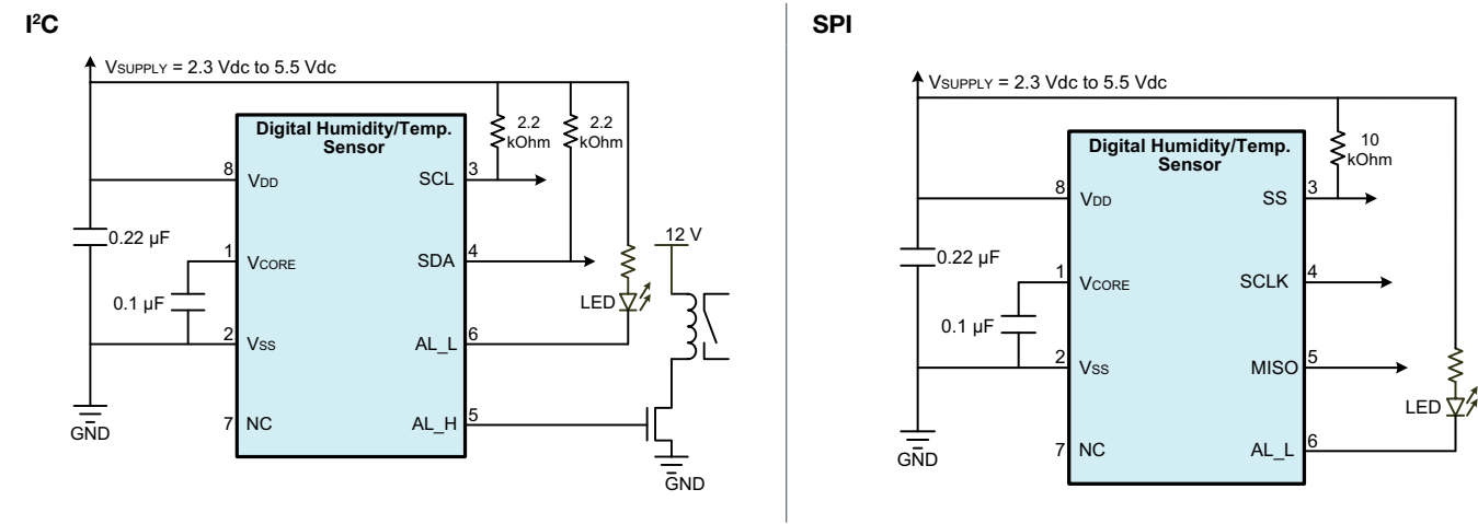
Figure 3. SOIC-8 SMD Typical Application Circuits
