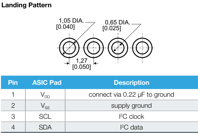
Figure 6. SIP 4 Pin Mounting Dimensions, PCB Landing Pattern and Pinout [For reference only: mm/[in].]
