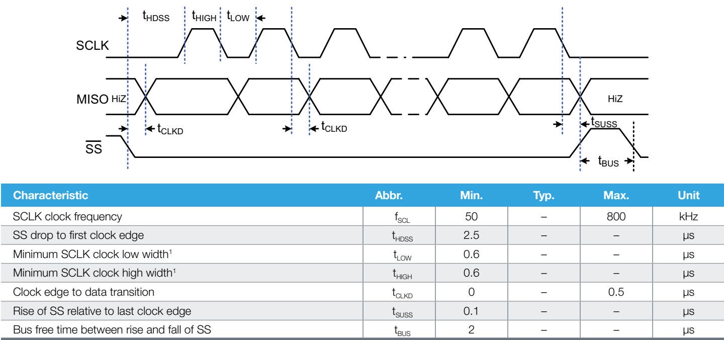
Figure 2. SPI Timing Diagram
