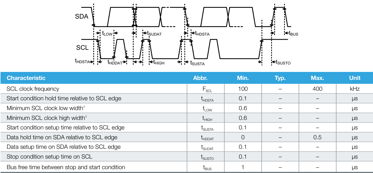
Figure 1. I 2 C Timing Diagram
