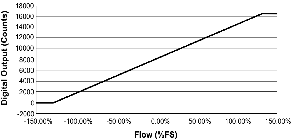
Figure 2. Nominal Digital Output
