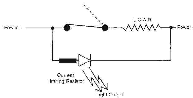
Figure 18. Wiring Diagram 3
