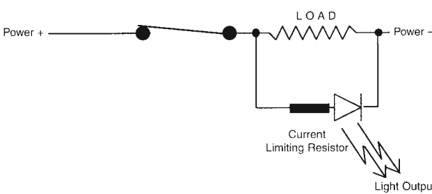
Figure 19. Wiring Diagram 4
