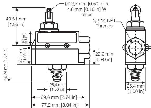
Figure 23. Cross roller plunger, reset, side mount
