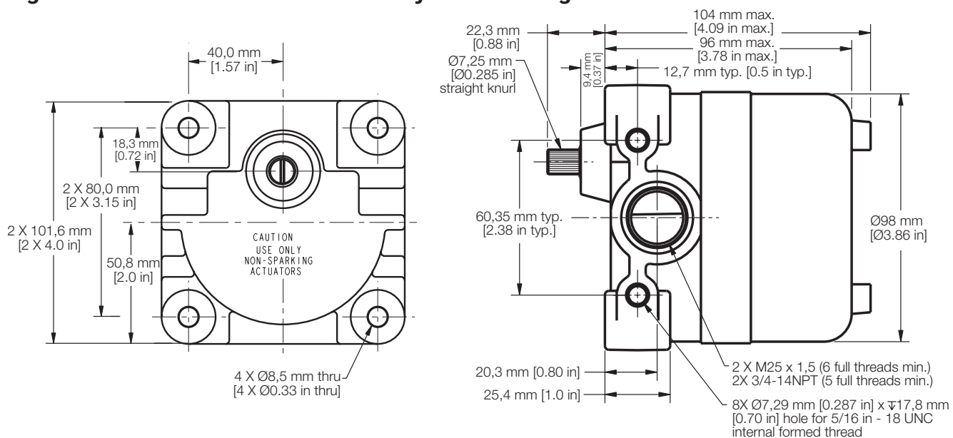
Figure 2. MICRO SWITCH CX - side rotary short housing
