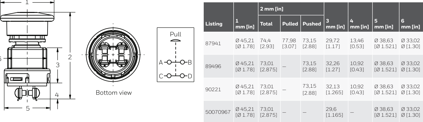
Figure 2. Push-pull/E-stop switches with 2NC circuitry and screw terminal
