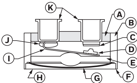
A Glass header B Housing C Contact D Movable contact E Actuator F Laser weld G Bimetallic disc H Cap I Contact arm J Weld cap K Terminals
