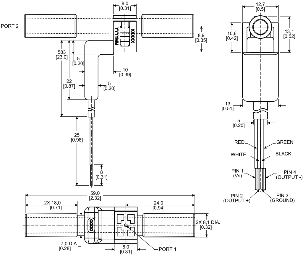
Figure 4. Pressure Port Types and Termination Configuration Dimensions (continued)
