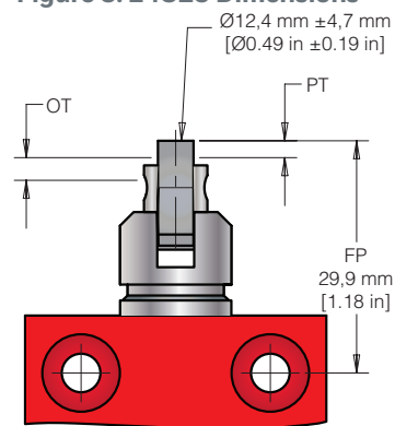
Figure 5. 24CE3 Dimensions
