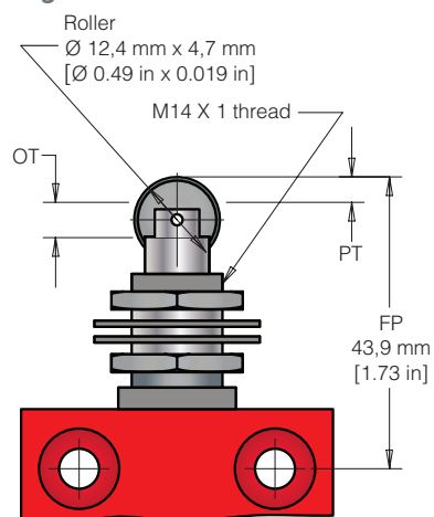
Figure 8. 24CE28 Dimensions
