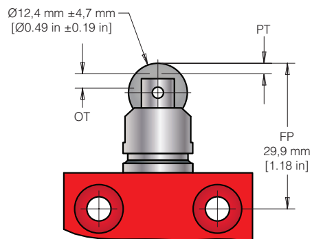
Figure 4. 24CE2 Dimensions
