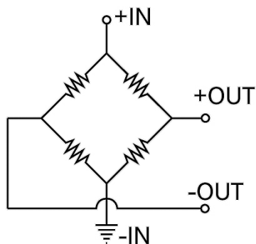
Figure 1. 13 mm Compensated Series
