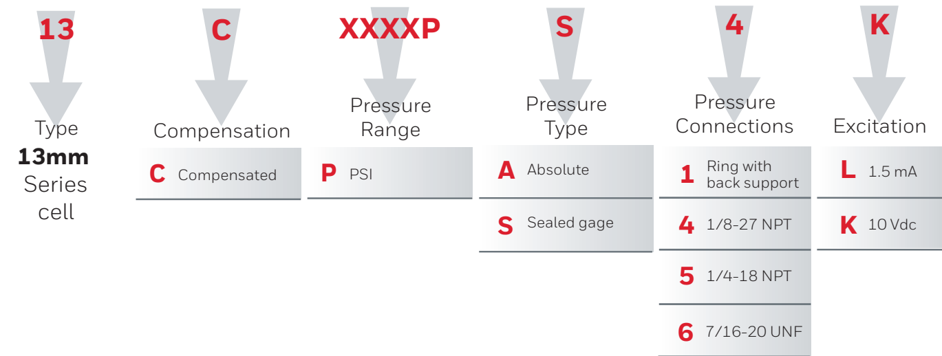
Figure 7. 13 mm COMPENSATED Series Product Nomenclature
