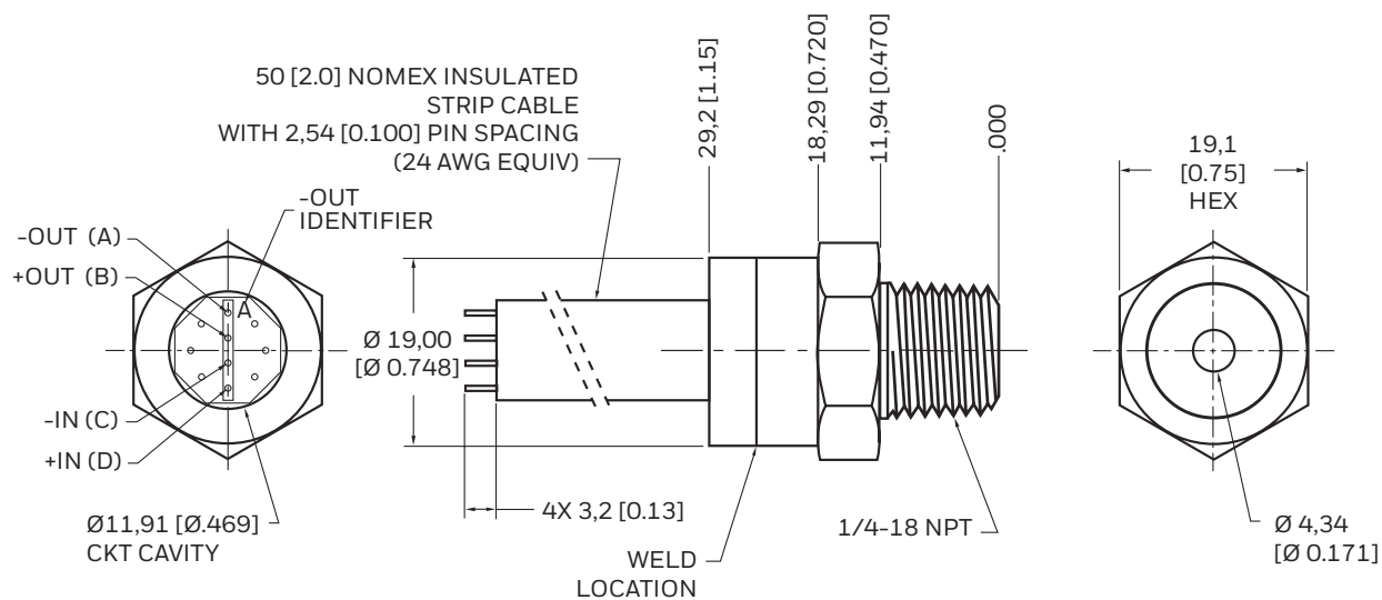
Figure 4. Package 5: 1/4-18 NPT
