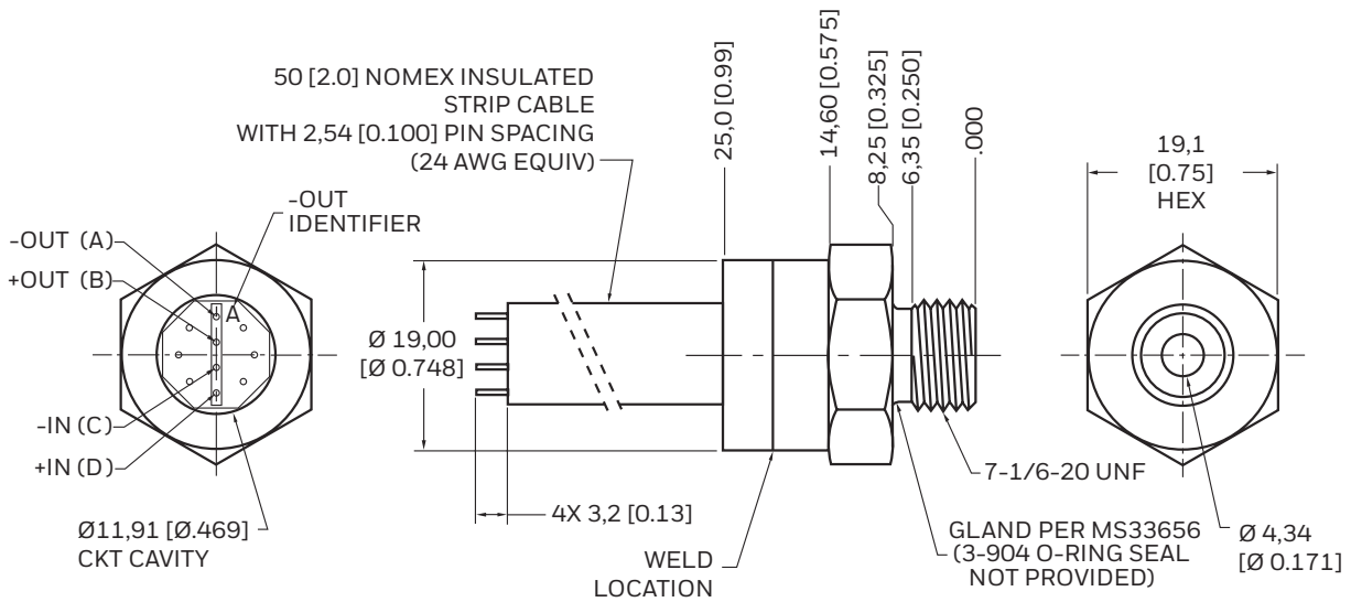
Figure 5. Package 6: 7/16-20 UNF
