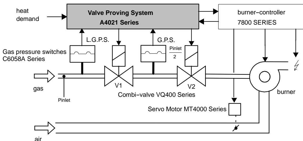
Fig. 4. System set-up .
