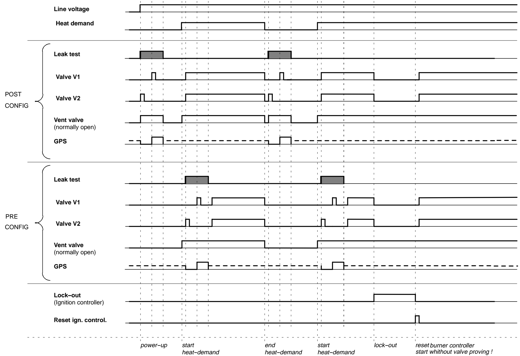
Fig. 6. System sequence of A4021A in post and pre-configuration.
