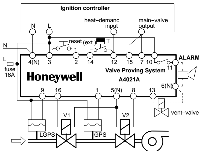
Fig. 10. Wiring diagram for 2-valve configuration pre-configuration
