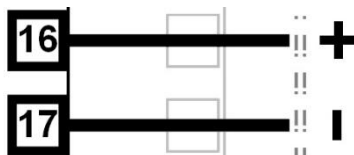
Figure 38. Plug-in Module Slot A – Basic Auxiliary Input Module
