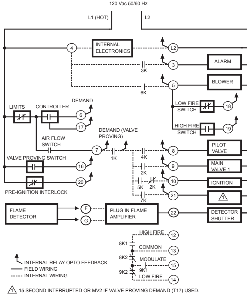
Fig. 2. Internal block diagram of the RM7800L/40L, EC7840L (See Figs. 3, 4, 6 or 7 for individual detailed wiring instructions).
