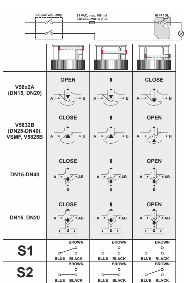
Fig. 10. Electric wiring of auxiliary switch
