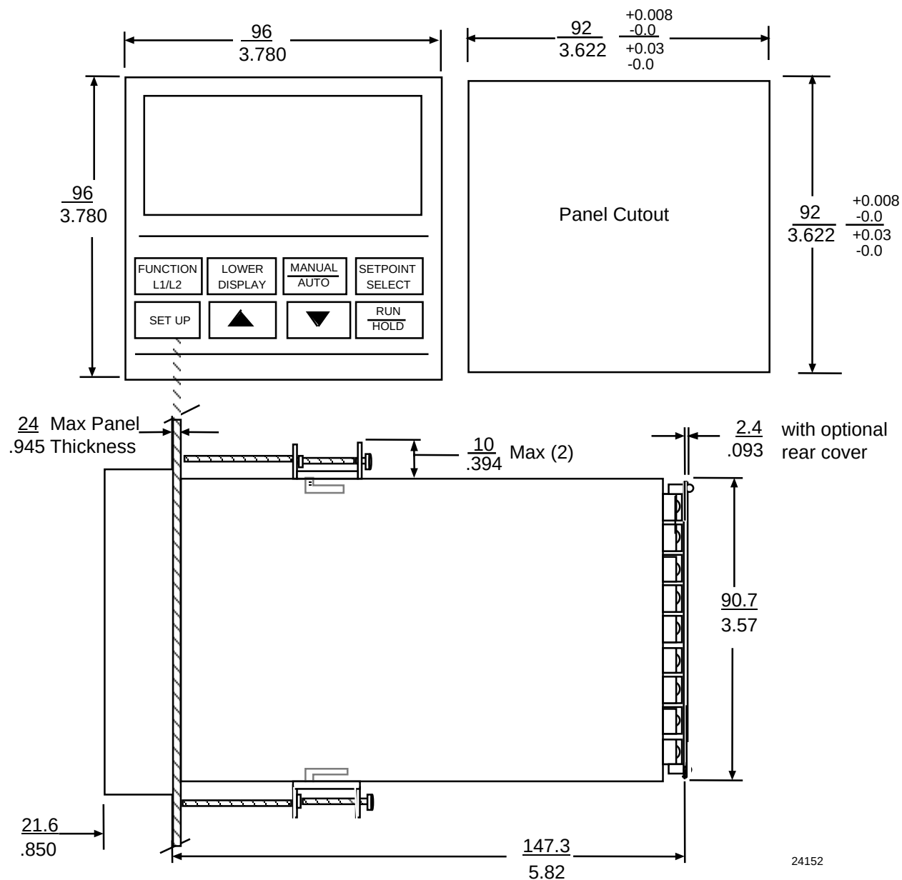
Figure 2-1 Dimensions
