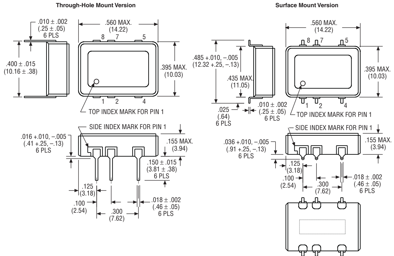
Figure 7 - Outline Dimensions
