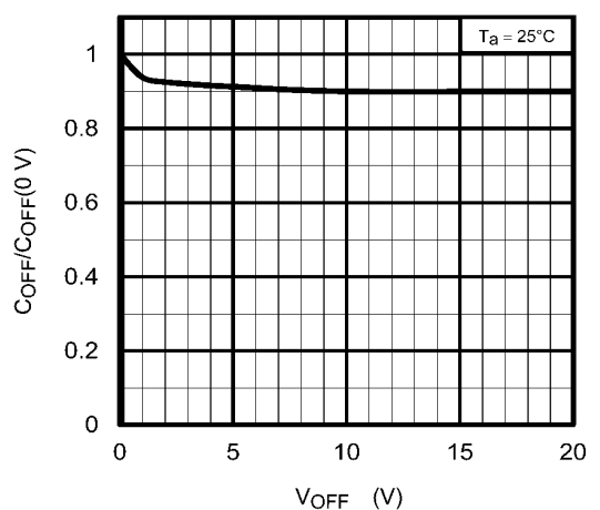
Fig. 12.1.11 C_{OFF}/C_{OFF}(0V) - V_{OFF}
