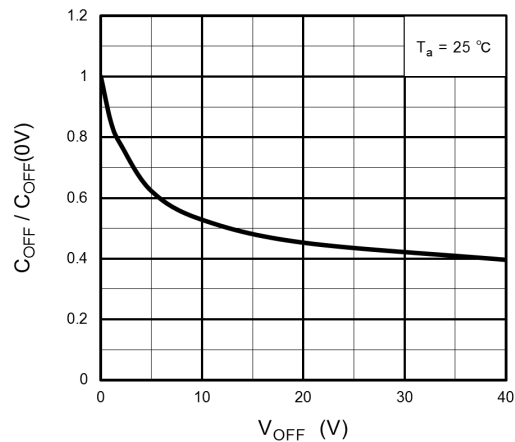
Fig. 12.1.10 C_{OFF}/C_{OFF}(0V) - V_{OFF}
