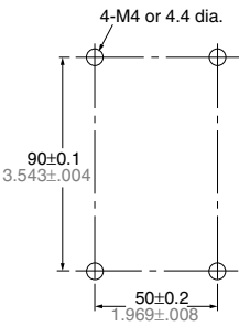
Mounting dimensions (Bottom view)
