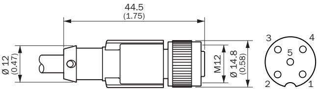
female connector M12 x1, straight, screened
