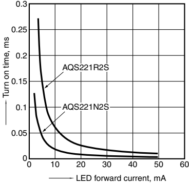
11. Turn on time vs. LED forward current characteristics Load voltage: 10 V (DC); Continuous load current: 160 mA (DC) R type 20 mA (DC) C type Ambient temperature: 25°C 77°F
