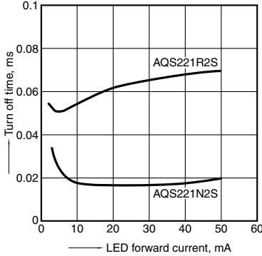
12. Turn off time vs. LED forward current characteristics Load voltage: 10 V (DC); Continuous load current: 160 mA (DC) R type 20 mA (DC) C type Ambient temperature: 25°C 77°F
