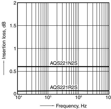
15. Insertion loss vs. frequency characteristics (50Ω impedance) Ambient temperature: 25°C 77°F
