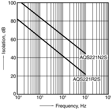
14. Isolation vs. frequency characteristics (50Ω impedance) Ambient temperature: 25°C 77°F
