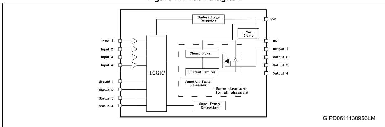
Figure 1. Block diagram
