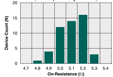
Typical On-Resistance Distribution (N=50, I_F=5\text{mA} , I_L=250\text{mA} )
