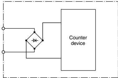
AC Supply
