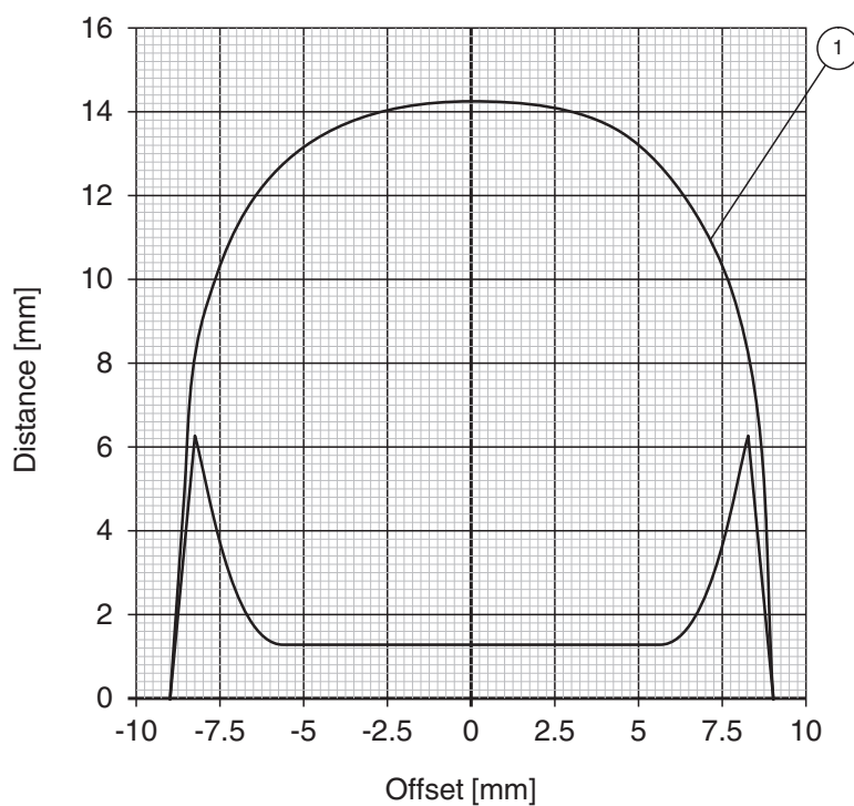
Reading range in air IQC21-12.4
