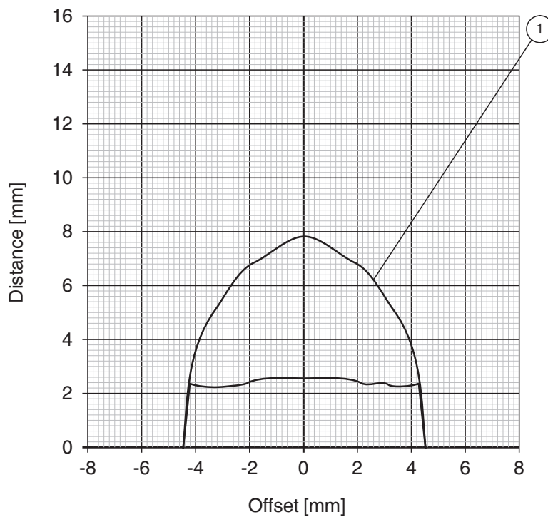
Reading range in steel IQC21-10
