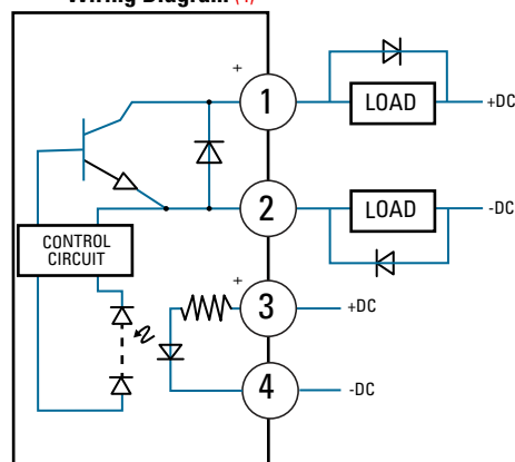
Wiring Diagram (4)
