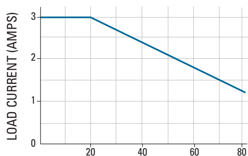
DMO Max. Load Current vs. Temp
