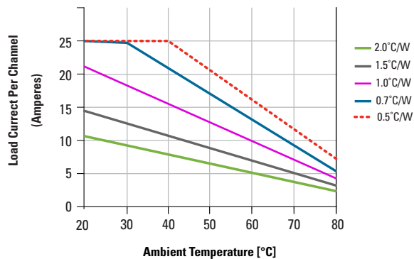
DERATE CURVES:
