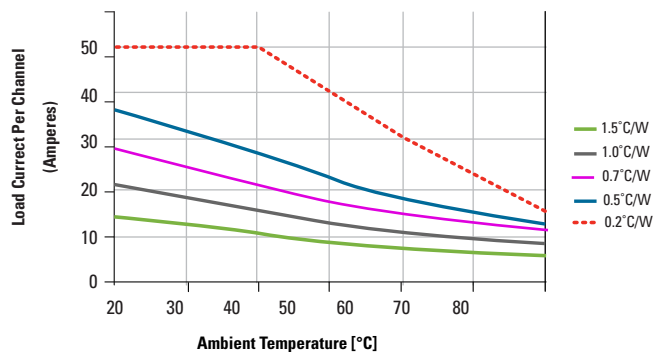
DERATE CURVES:
