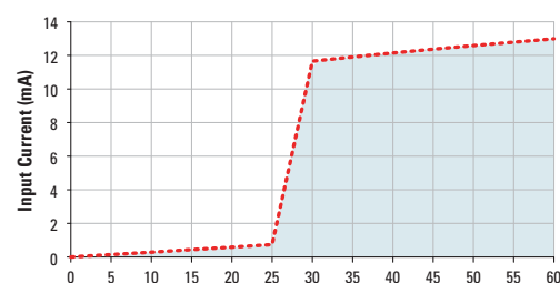
Input Current vs Input Voltage DC500F60
