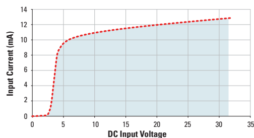
Input Current vs Input Voltage DC500D60
