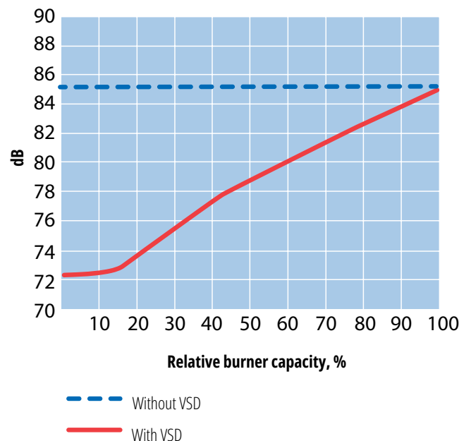
Noise level with VSD and without VSD
