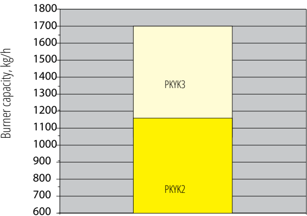
Diagram 1 Selection of a booster unit for light fuel oil
