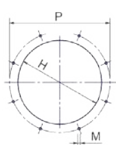
BOILER RECOMMENDED DRILLING TEMPLATE
