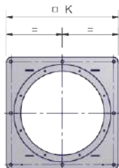
BURNER FLANGE
