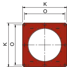
BURNER FLANGE
