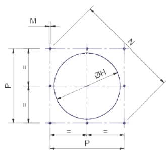
BOILER RECOMMENDED DRILLING TEMPLATE
