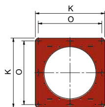
BURNER FLANGE
