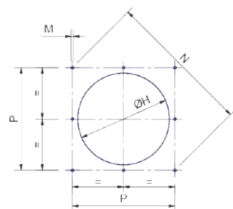
BOILER RECOMMENDED DRILLING TEMPLATE
