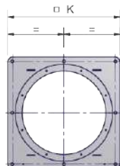
BURNER FLANGE
