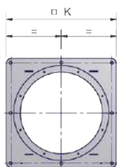
BURNER FLANGE
