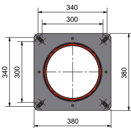
BURNER FLANGE
