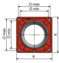
BURNER FLANGE
