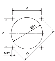
BOILER RECOMMENDED DRILLING TEMPLATE
