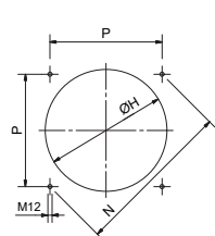
BOILER RECOMMENDED DRILLING TEMPLATE
