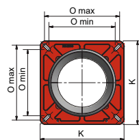
BURNER FLANGE
