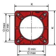
BURNER FLANGE
