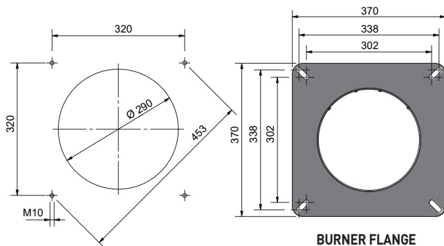
BOILER RECOMMENDED DRILLING TEMPLATE
