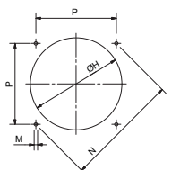
BOILER RECOMMENDED DRILLING TEMPLATE
