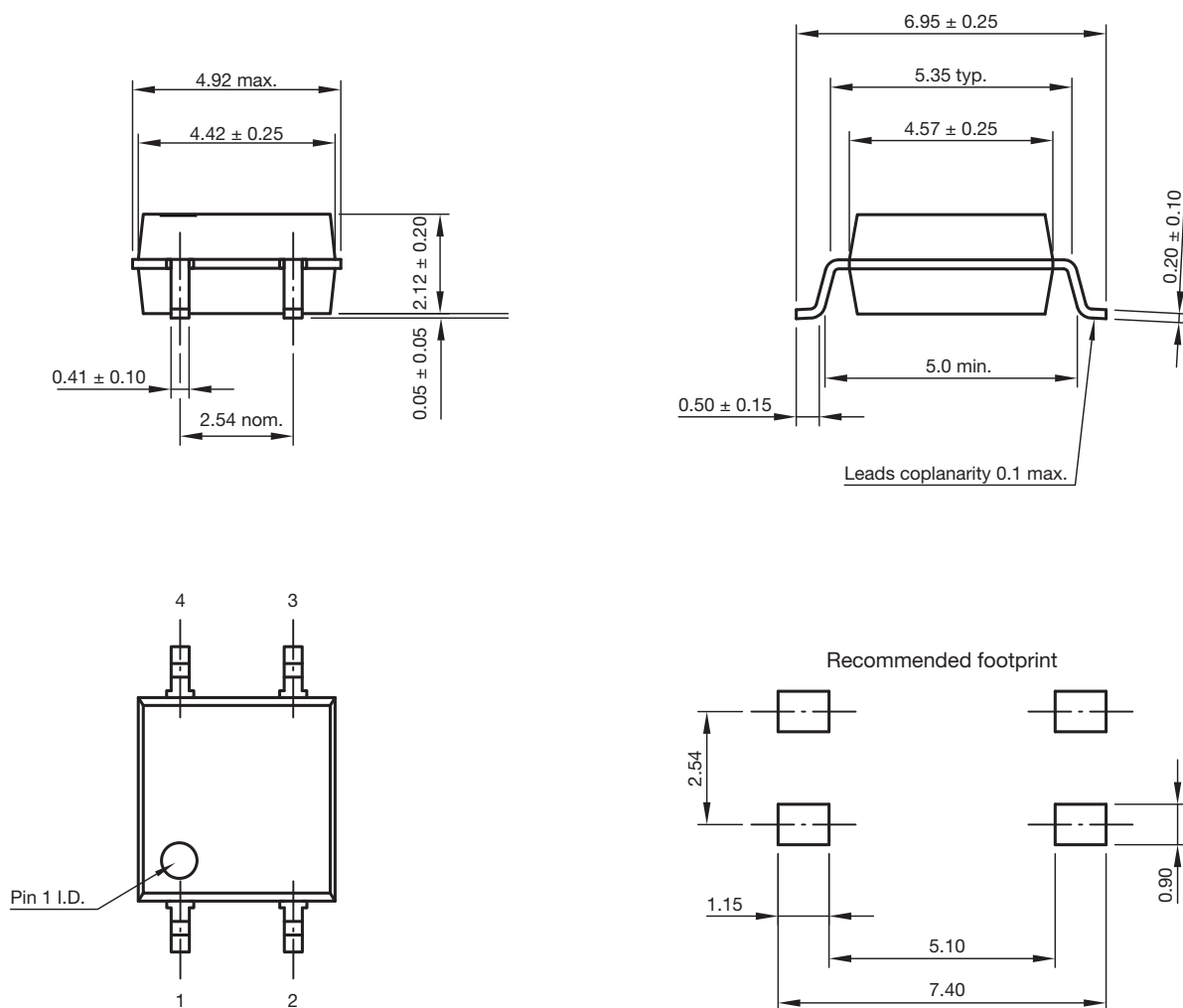
Fig. 15 - Package Drawing
