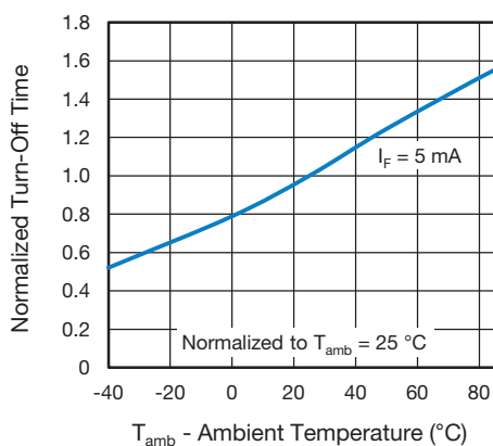
Fig. 14 - Normalized Turn-Off Time vs. Ambient Temperature
