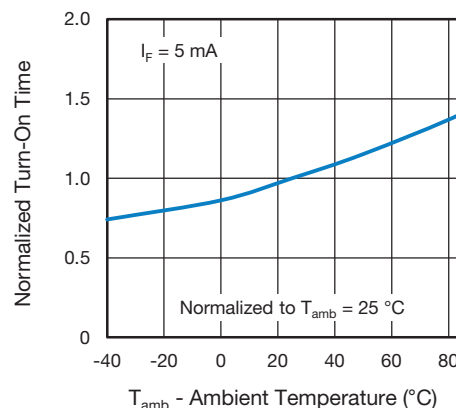
Fig. 7 - Normalized Forward Current for Switch Turn-On vs. Ambient Temperature
